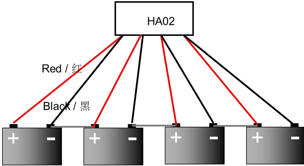
4*12V battery bank
